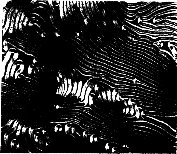
FIG. 153.—Elongated "Liquid Crystals" of Dibenzal Benzidine, showing Double Refraction and Dichroism
